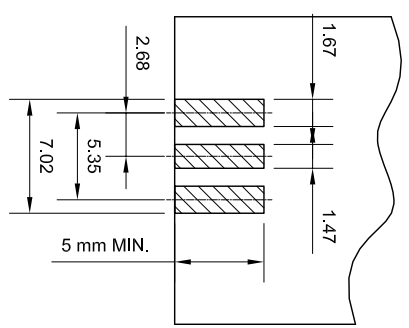
LANDING PAD DIMENSIONS
