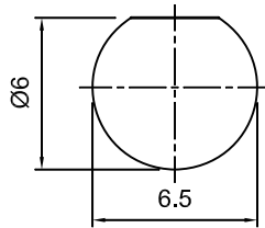
MOUNTING HOLE CUTOUT
